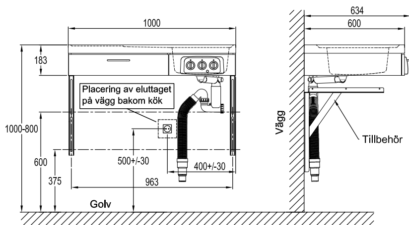
Trinette special 1000 mm ETN1083, ETN1084
