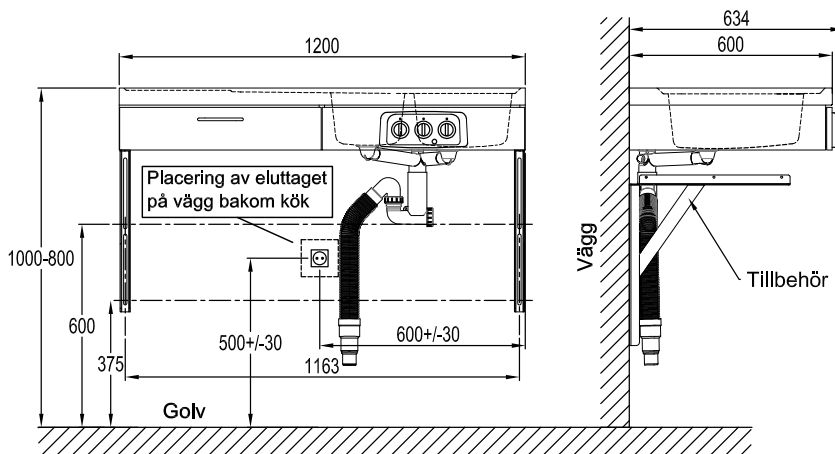
Trinette special 1200 mm ETN1283, ETN1284
