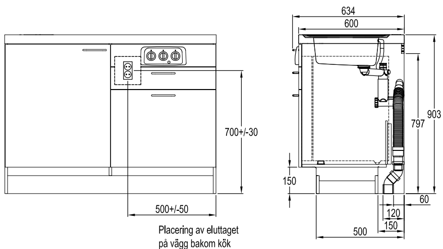
Trinette 1200 mm ETN1250, ETN1254, ETN1264
